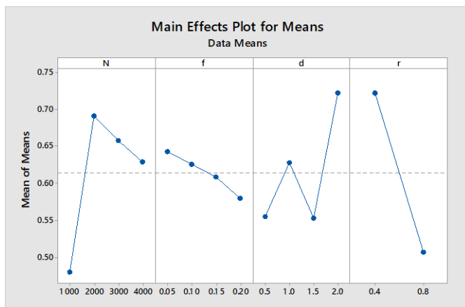
Fig. 1 Main Effect Plots for Means of Composite Relative Distance
