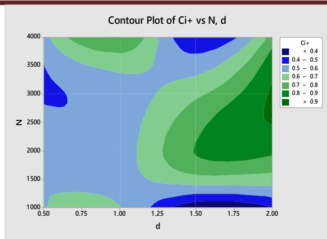
Fig. 4: Contour Plot of C_i^+ Vs N, d
